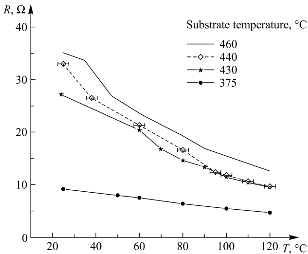
Fig. 3. Temperature dependence of resistance ( R )
