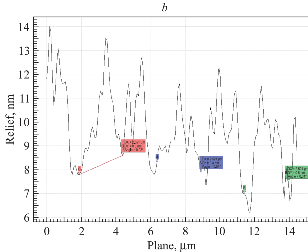
Fig. 3. Surface morphology of a sample (AFM): a – surface morphology of the exposed sample 3D; b – profile of the surface structure
