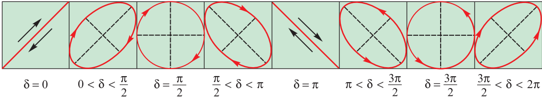
Fig. 2. Polarisation of optical field
