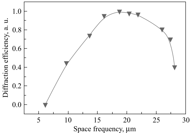
Fig. 5. Dependence of diffraction efficiency on spatial frequencies
