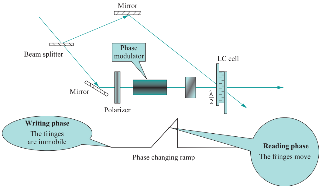
Fig. 6. Experimental set-up for moving grating measurement
