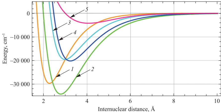
Fig. 5. Potential energy curves of the ground state of the RaF (1), RaCl (2), RaBr (3), RaI (4) and KRb (5) molecules
