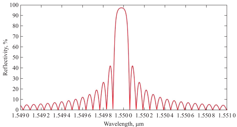
Fig. 2. Reflectivity of a uniform periodic fiber gratings with number of periods N = 22\ 620 and \Delta n_{co} = 0.000\ 1 , leading to a total reflection 97 % with narrow central peak wavelength 1550 nm
