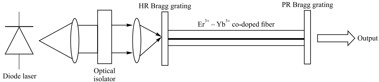
Fig. 5. Schematic diagram of the \text{Er}^{3+} - \text{Yb}^{3+} co-doped fiber laser
