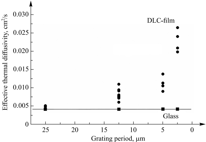
Fig. 1. Effective thermal diffusivity of the system diamond-like carbon film – glass as a function of the period of a thermal transient grating formed on surface of the absorbing film of thick 2 μm
