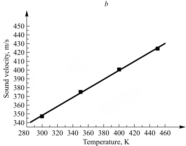
Fig. 3. PbTe : Bi film: Fourier spectrum of the diffracted signal for PbTe : Bi film (vertical line denotes the component of acoustic oscillations in air at frequency 8.32 MHz) ( a ) and temperature dependence of the ultrasonic speed in air (■ is reference points [16]) ( b )
