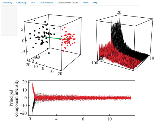
Fig. 5. FluorSimStudio web application interface windows: examples of simulation modelling the stretched-exponential fluorescence decay dataset ( a ) and analysis results visualisation ( b ) of clustered fluorescence decay curves
