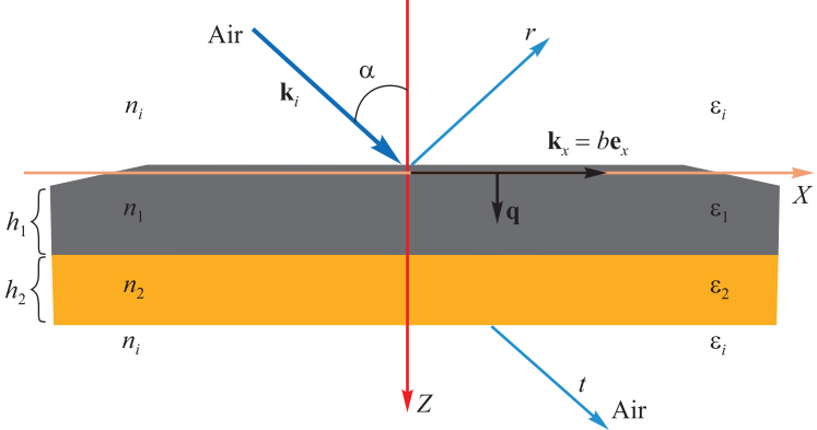
Fig. 2. Schematic of the wave reflection and transmission
