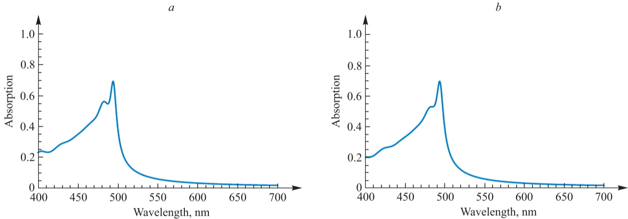
Fig. 4. Absorption spectrum of the HMM composition (AB)_{70} (a) and absorption spectrum of the hypercrystal composition ((AB)_{10}C)_7 (b). Dielectric (A) and metal (B) have the same thicknesses 4.5 nm, while the dielectric spacer is 10 nm thick
