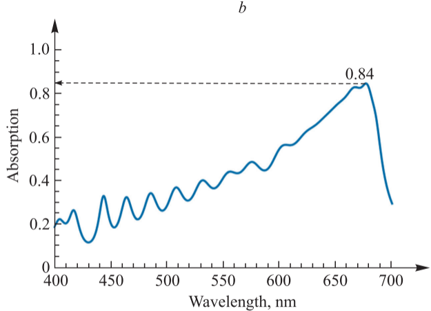
Fig. 6. Absorption spectrum of the hypercrystals ((AB)_{10}C)_7 ( a ) and ((AB)_{20}C)_7 ( b ) (dielectric and metal of 6 and 3 nm thickness, air spacer thickness 10 nm)
