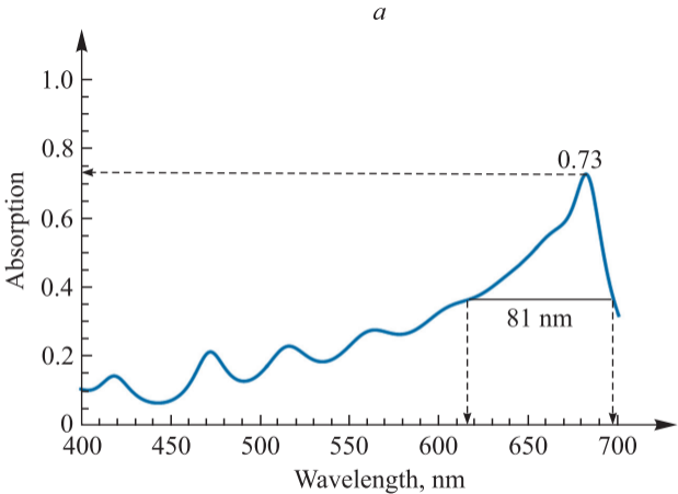
Fig. 6. Absorption spectrum of the hypercrystals ((AB)_{10}C)_7 ( a ) and ((AB)_{20}C)_7 ( b ) (dielectric and metal of 6 and 3 nm thickness, air spacer thickness 10 nm)
