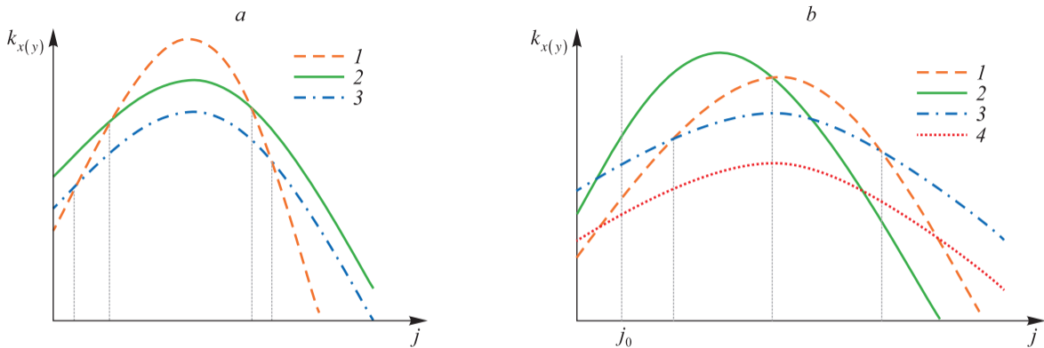
Fig. 1. The relative position of the k_x (1) and k_y (2–4) curves with increasing temperature to explain the results of [27] (a) and [30] (b). Remember, that k_y = k_y(T) and T_2 < T_3 < T_4 , where the temperature index corresponds to the number of the curve
