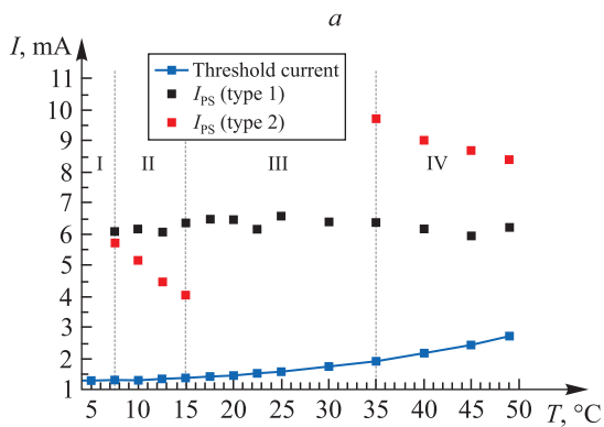
Fig. 2. Temperature dependence of PS points of different types according to the results of experimental studies by the authors [9; 34] (a); qualitative behaviour of the roots j_{p1} and j_{p2} in the region of the formal extinction of j_{p2} (b). The range of valid values for PS points is shaded
