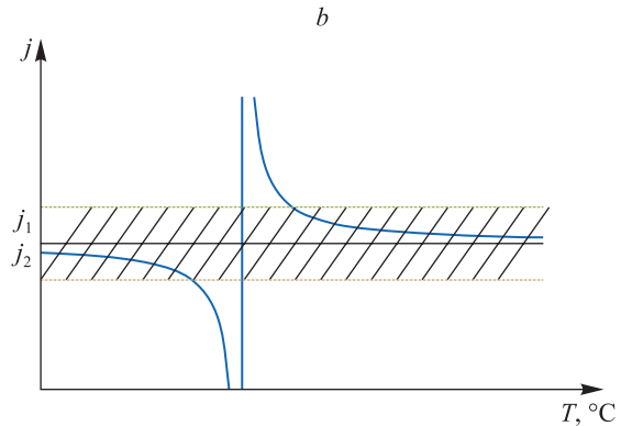
Fig. 2. Temperature dependence of PS points of different types according to the results of experimental studies by the authors [9; 34] (a); qualitative behaviour of the roots j_{p1} and j_{p2} in the region of the formal extinction of j_{p2} (b). The range of valid values for PS points is shaded
