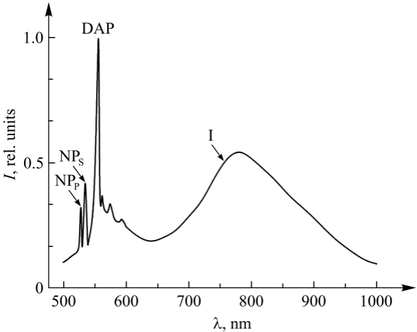
Fig. 1. PL spectra of standard GaP epitaxial layers at T = 4.2 K
