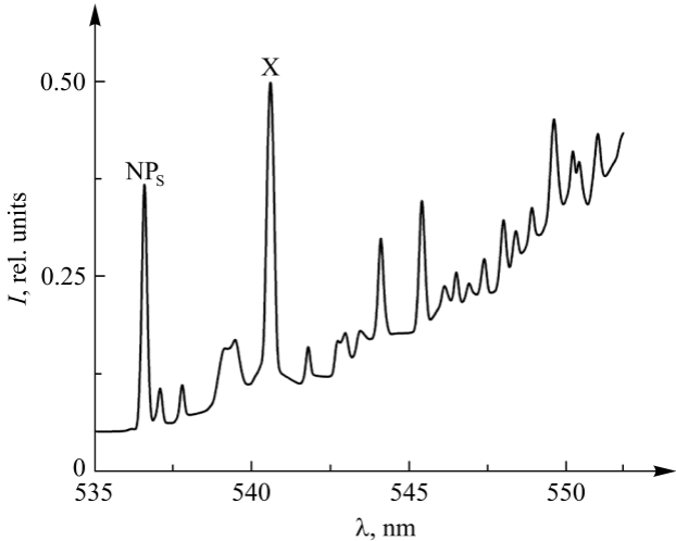
Fig. 4. PL spectra at T = 4.2 K of GaP : REE epitaxial layers obtained from melt-solutions with REE content of 0.2 wt. %, as well as ultrapure films obtained from the melt subjected to high-temperature heat treatment
