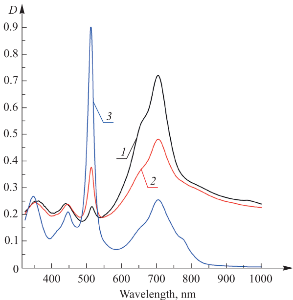
Fig. 3. Absorption spectra of the dye 2 aqueous suspensions 3 min (1) and 30 min (2) after ultrasonication; absorption spectrum of the dye 2 aqueous solution decanted 14 days after ultrasonication (3)
