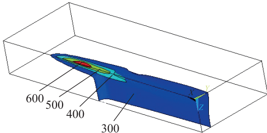
Fig. 2. Temperature distribution in the volume of the processed plate, K
