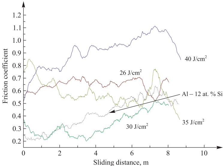
Fig. 7. Dependence of the friction coefficient on the indenter sliding distance for the sample of Al – 12 at. % Si alloy and samples of (Ti, Cu)N/Al – 12 at. % Si treated by CPF with different absorbed energy density
