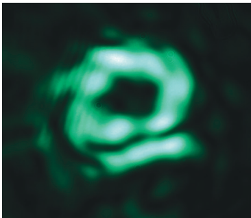
Fig. 1. Photo of the vortex beam ( a ) and the result of numerical modelling of the singular beam profile ( b )
