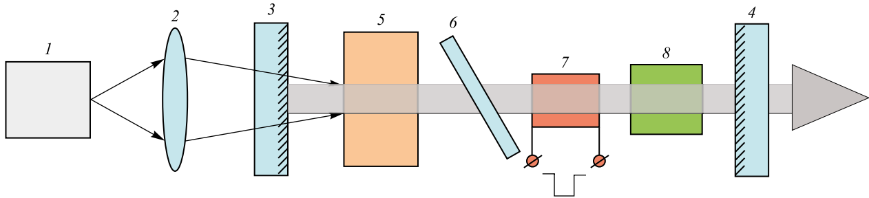
Fig. 1. Setup for the cavity dumping by the second harmonic generation in the actively Q-switched laser: 1 – diode laser; 2 – lens; 3, 4 – resonator mirrors; 5 – laser crystal; 6 – polarizer; 7 – electro-optical crystal; 8 – second harmonic crystal
