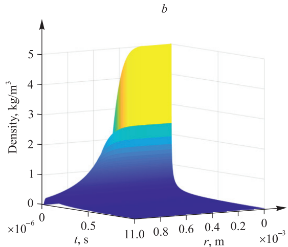
Fig. 2. Spatial-temporal distributions of pressure ( a ) and density ( b ) of silver vapor inside the jet
