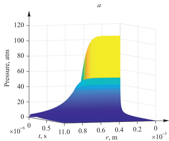
Fig. 2. Spatial-temporal distributions of pressure ( a ) and density ( b ) of silver vapor inside the jet
