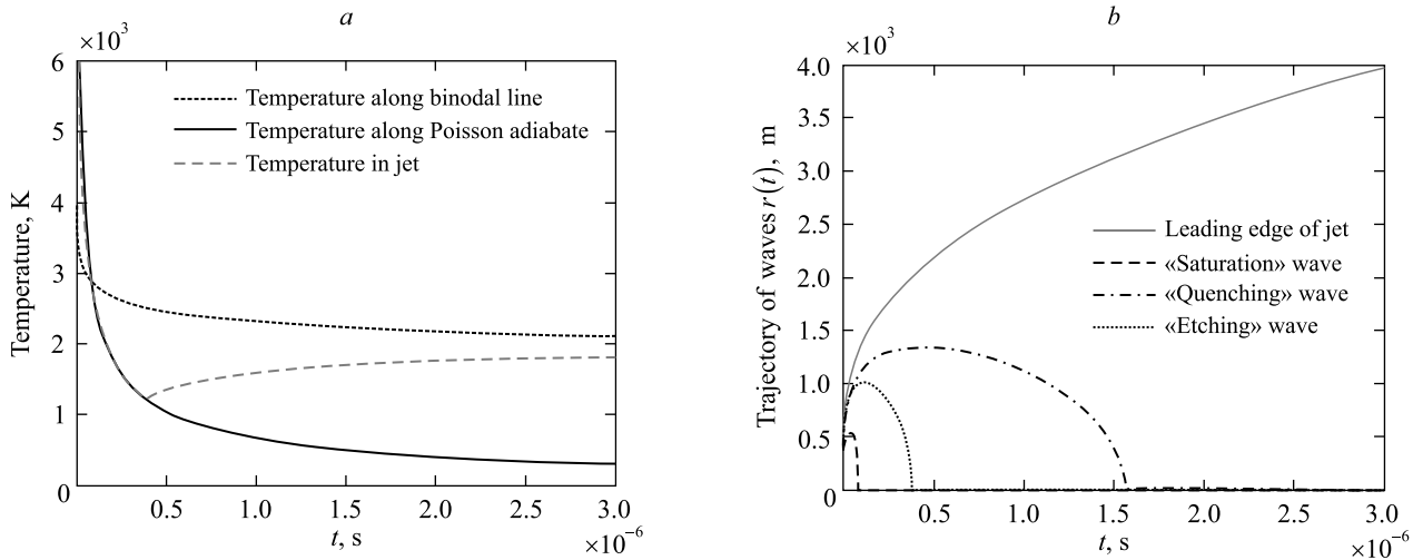
Fig. 3. Dynamic condensation in silver jets: a – temperature dynamics in the center of the silver ablation jet ( \xi = 0 ); b – wave fronts of dynamic condensation
