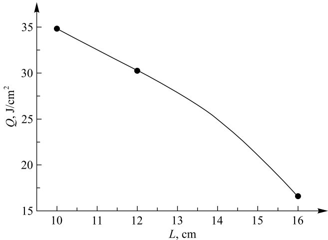
Fig. 1. Dependence of the absorbed energy density in the surface layer of aluminum on the distance between the sample and electrode during the CPF impact ( U = 4.0 \text{ kV} )
