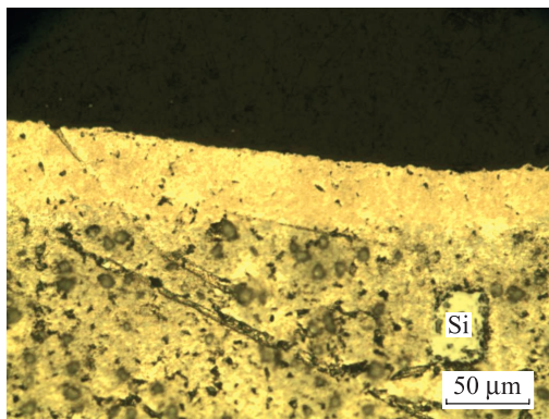
Fig. 2. Optical images of the cross-sections of the samples of Al – 20Si alloy after CPF impact at U = 4.0 kV and L is equal 14 cm (a), 10 cm (b), 6 cm (c).
