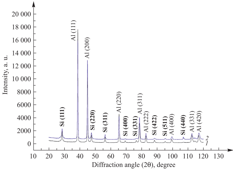
Fig. 4. XRD patterns of the Al – 20Si alloy after the CPF impact at U = 3.0 kV and L is equal 14 cm (1), 6 cm (2)
