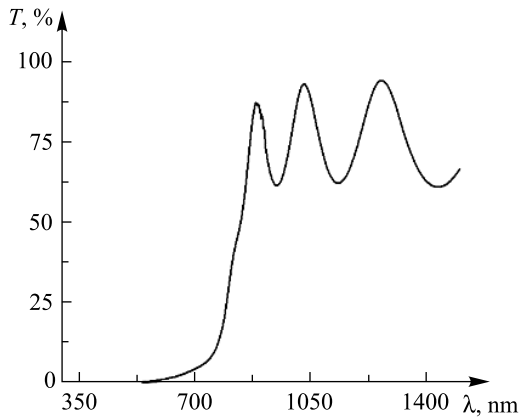
Fig. 1. Transmission spectrum of CdTe thin film
