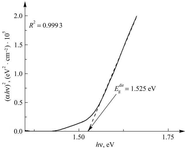
Fig. 5. Absorption coefficient \alpha in presentation of (\alpha h\nu)^2 as function of photon energy h\nu : R^2 is the coefficient of determination; E_g^{\text{dir}} is the direct bandgap
