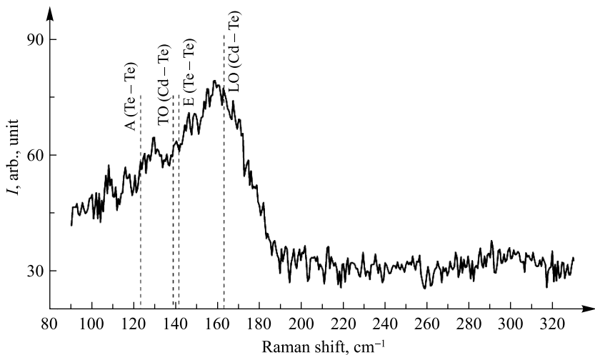
Fig. 6. Raman spectra of CdTe thin film: laser excitation wavelength is \lambda = 514.532 \text{ nm} ; laser power is 1 mW; the exposure time is 60 s
