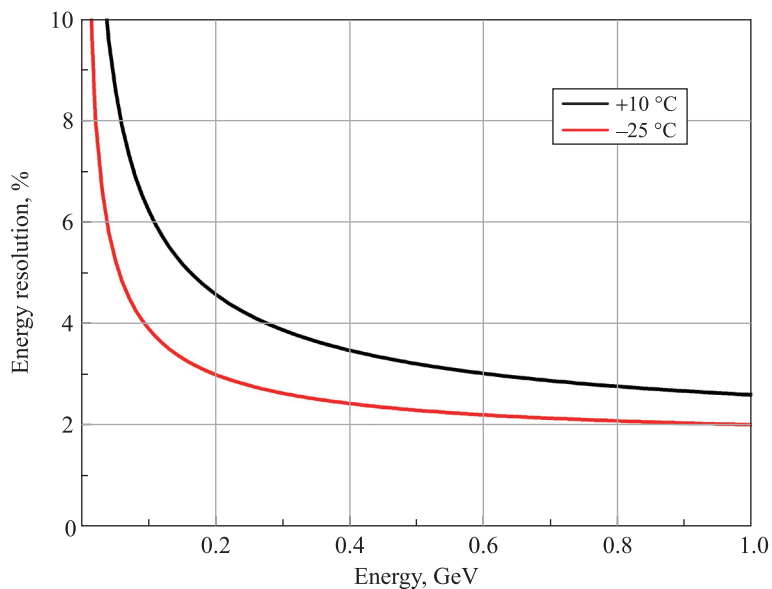
Fig. 2. The energy resolution of a 3 \times 3 PWO matrix of 200 mm long crystals measured at two different operating temperatures of -25 and +10\text{ }^{\circ}\text{C} , respectively (after [9])
