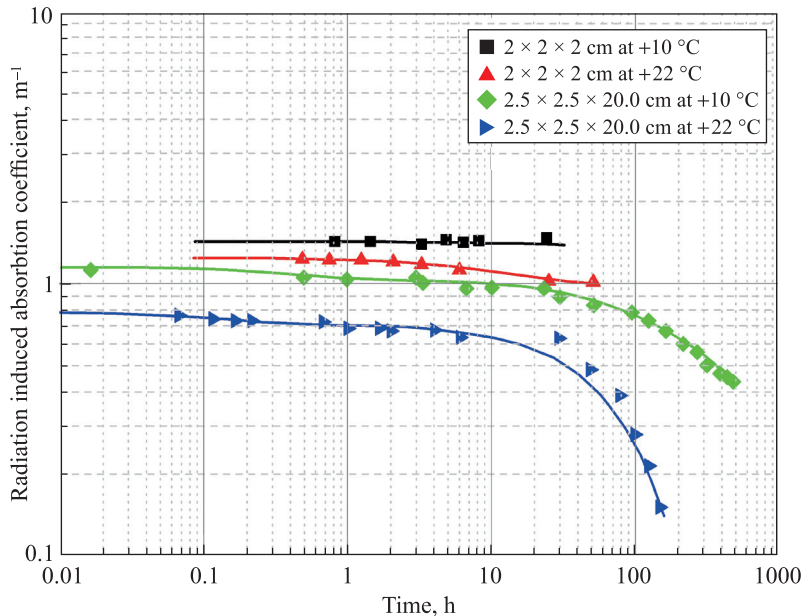
Fig. 3. Spontaneous recovery of the radiation induced absorbance coefficient at 420 nm of two PWO samples irradiated and measure at +22 and +10 °C. Samples are courtesy of the PANDA Collaboration at FAIR (Darmstadt)
