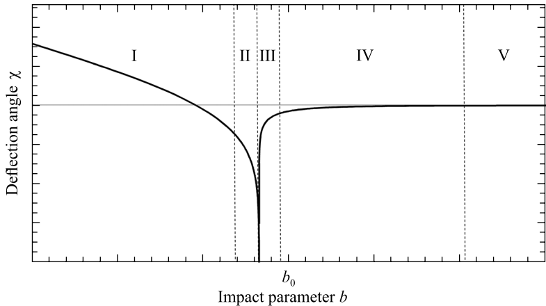
Fig. 6. The dependence of deflection angle \chi on impact parameter b : I–V are intervals
