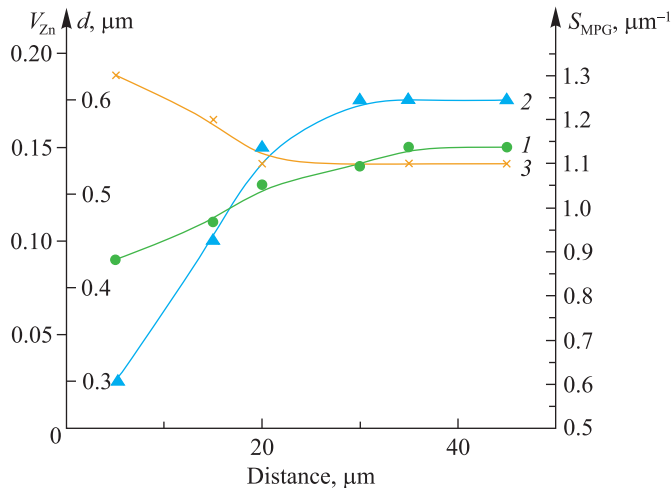
Fig. 3. Dependence of the volume fraction of zinc V_{\text{Zn}} (1), the average length of chords d_{\text{Zn}} (2) and the specific surface of S_{\text{MPG}} (3) of the Sn – 15 wt. % Zn alloy foil
