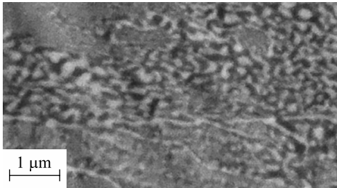
Fig. 4. Microstructure of foil layers adjacent to surface A for Sn – 60 wt. % Zn ( a ) and Sn – 80 wt. % Zn ( b )
