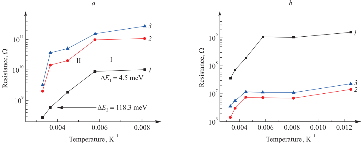
Fig. 5. Temperature dependences of the elements of the 1 st (a) and 2 nd (b) resonant RCL-circuits ( 1 - R_i , 2 - R_{Ci} , 3 - R_{Li} , i = 1, 2 ) of the (Fe_{0.45}Co_{0.45}Zr_{0.10})_{0.31}(Al_2O_3)_{0.69} nanogranular composite film, deposited in Ar – O 2 mixture, ESC. I – low temperature region, II – high temperature region
