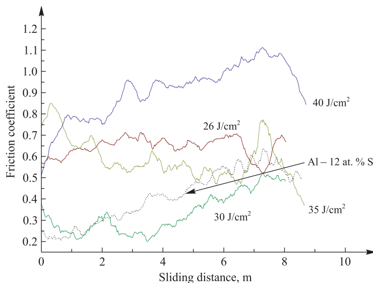
Fig. 7. Dependence of the friction coefficient on the indenter sliding distance for the sample of \text{Al} - 12 \text{ at. \% Si} alloy and samples of (\text{Ti}, \text{Cu})\text{N}/\text{Al} - 12 \text{ at. \% Si} treated by CPF with different absorbed energy density
