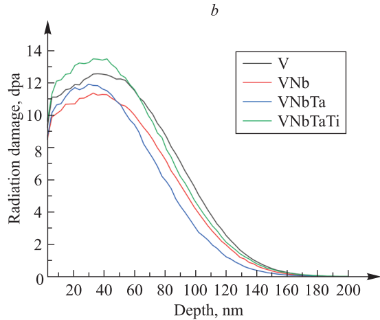
Fig. 1. Profiles of the distribution of implanted \text{Kr}^{14+} ion ( a ) and the damaging dose ( b ) in samples V, VNb, VNbTa, VNbTaTi by depth
