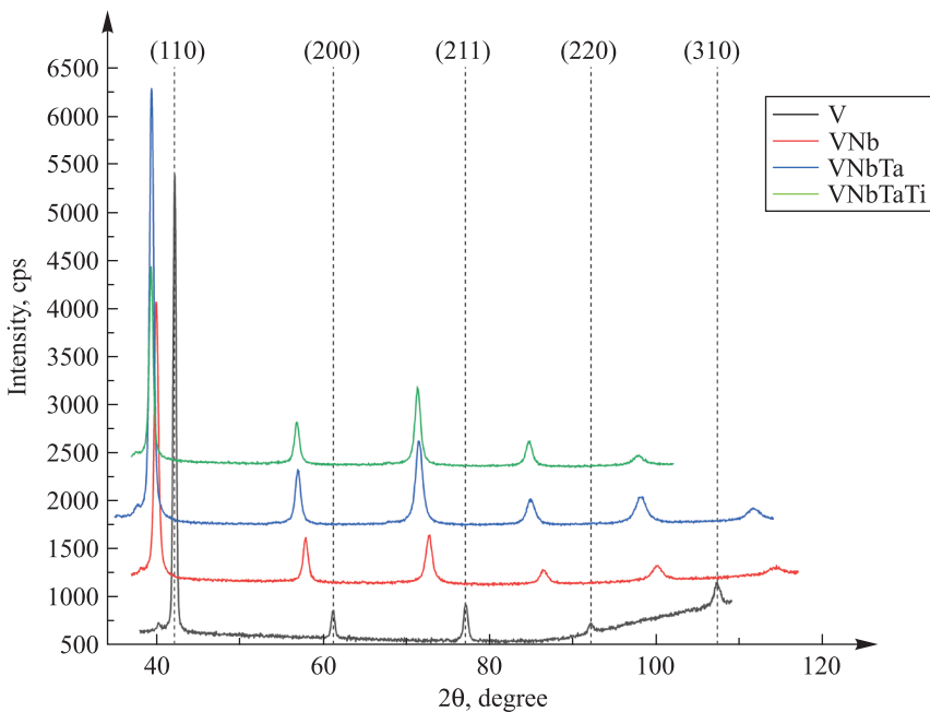
Fig. 5. X-ray diffraction pattern of samples of the V – Nb – Ta – Ti system irradiated by \text{Kr}^{14+} ions with an energy of 280 keV
