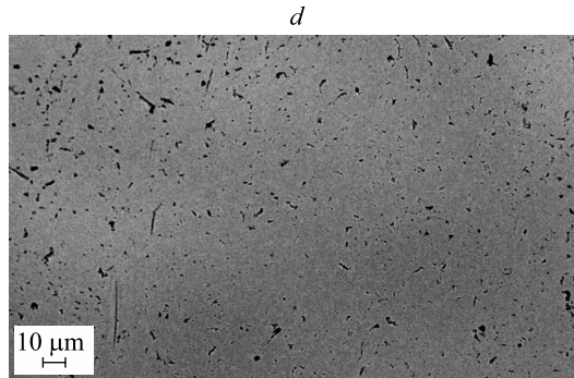
Fig. 6. Surface morphology in the samples surface V ( a ), VNb ( b ), VNbTa ( c ), VNbTaTi ( d ) irradiated by \text{Kr}^{14+} ions with an energy of 280 keV
