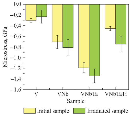
Fig. 8. Values of macrostresses (a) and microstresses (b) depending on the complexity of the composition of the V – Nb – Ta – Ti system for the initial and irradiated samples
